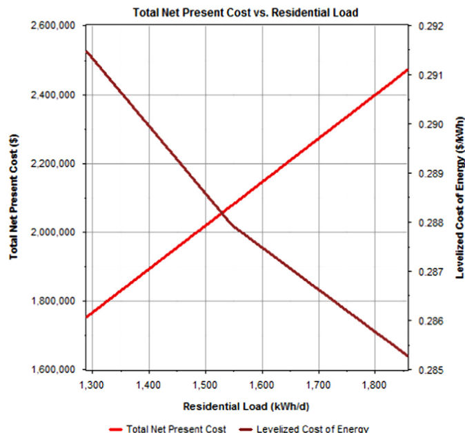
Fig. 14. A line graph showing the effect of increasing demand with respect to NPC and COE.
