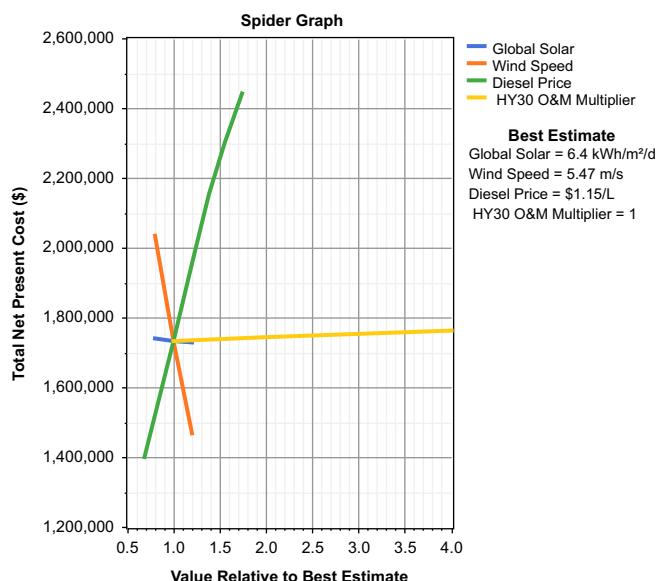
Fig. 13. The spider graph of the three sensitivity variables input into HOMER.
