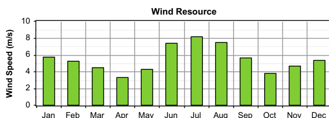
Fig. 3. Monthly averaged wind speed at Hargeisa.
